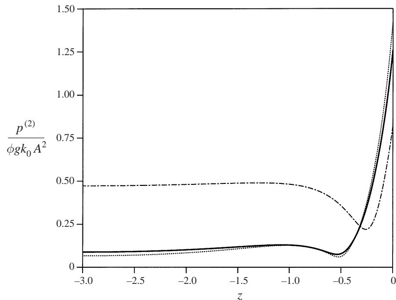
FIGURE 8. Distribution of the second-order pressure, |p^{(2)}|/\rho g k_0 A^2 , down the sides ( \theta_k = 0 ) of four cylinders, for a wave incidence \beta = 0 . Full line: results for isolated cylinder; dotted line: first and fourth cylinder; dot-dashed line: second and third cylinder.
